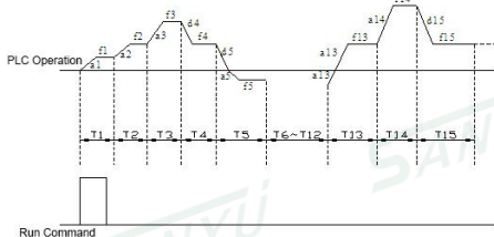
Fig.F9-2 Maintain Last Stage after Single Cycle
