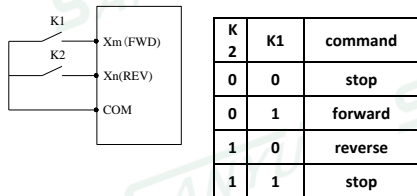
Fig. F7-2 2-wire Control Mode 1
