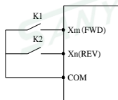
Fig. F7-3 2-wire Control Mode 2
