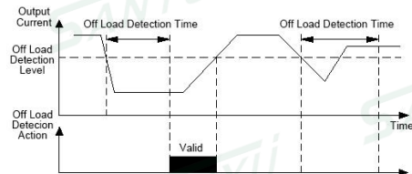
Fig. FA-3 Off Load Detection
