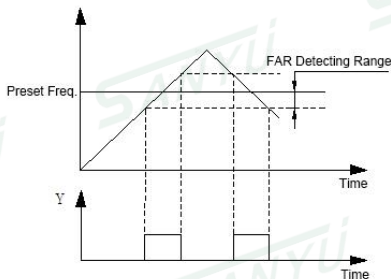
Fig. F7-7 Frequency Arrival
