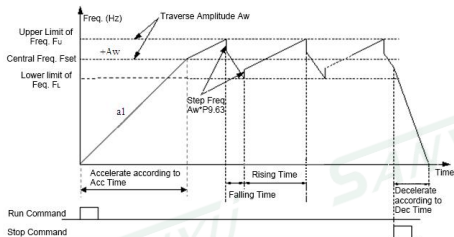
Fig.F9-6 Traverse Operation
