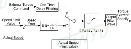
Figure F4-2 Torque Control Simplified diagram
