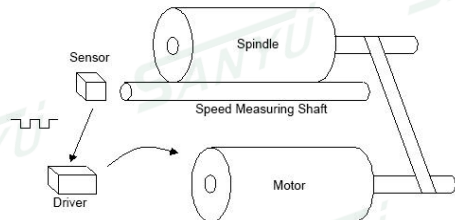
Fig. F9-7 Application of Stop at Fixed Length
