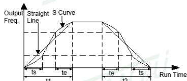
Fig. F1-3 Straight Line and S Curve of Acc./Dec.
